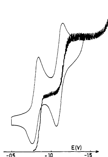
Figure 9. CV on platinum and polarography at the DME of \text{Zn}(\mathbf{1})_2^{2+} in 0.1 mol \text{L}^{-1} \text{CH}_2\text{Cl}_2 -TBAP (scan rate for CV, 40 mV \text{s}^{-1} ; E versus \text{Ag}/\text{Ag}_3\text{I}_4 ).
