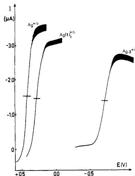
Figure 8. Polarography at the DME of \text{Ag}^+ , \text{Ag}(\mathbf{1})_2^+ , and \text{Ag}\cdot 2^+ in 0.1 mol \text{L}^{-1} \text{CH}_3\text{CN} -TEAP ( E versus SCE).
